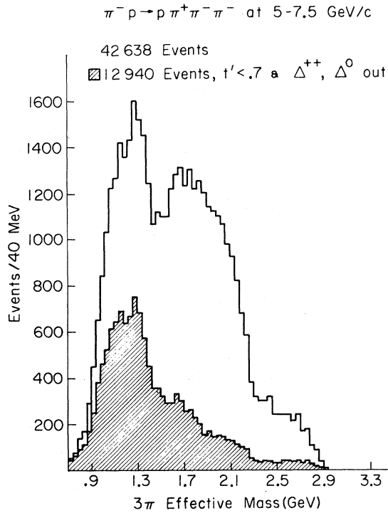
FIG. 2. \pi^+ \pi^- \pi^- mass spectrum for the 5-7.5-GeV/c data. The shaded histogram is for t' < 0.7 \text{ GeV}^2 , M_{p\pi^+} < 1.4 \text{ GeV} out, M_{p\pi^-} = 1.16-1.32 \text{ GeV} out.
