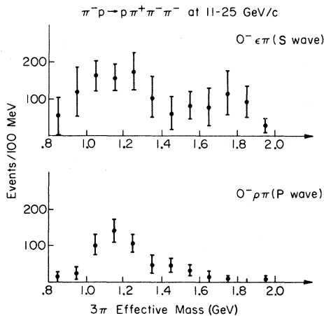
FIG. 15. Contributions of 0^-(S \rightarrow \epsilon\pi) and 0^-(P \rightarrow \rho\pi) vs M_{3\pi} for 11–25-GeV/c ( t' < 0.7 \text{ GeV}^2 ) data.
