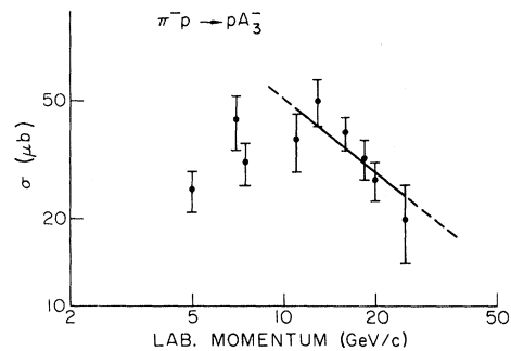
FIG. 23. Cross section for \pi^-p \rightarrow A_3^-p vs incident momentum. The cross sections refer only to the production of \pi^+\pi^-\pi^- with M_{3\pi} = 1.5-1.8 GeV and t' < 0.7 GeV ^2 through the amplitude 2^-(S \rightarrow f^0\pi^- \rightarrow \pi^+\pi^-\pi^-) .
