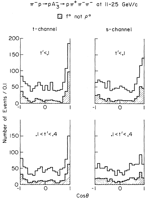
FIG. 22. \cos\theta distributions for events in M_{3\pi} = 1.5-1.8 GeV, M_{p\pi^+} = 1.16-1.32 GeV out, for 11-25-GeV/c data. Distributions are shown for the t -channel frame ( \cos\theta = \hat{n}_{in} \cdot \hat{n}^+ in 3-\pi frame) and in the s -channel frame ( \cos\theta = -\hat{p}_{out} \cdot \hat{n}^+ in 3-\pi frame) for the intervals t' < 0.1 GeV ^2 and t' = 0.1-0.4 GeV ^2 . The shaded distributions are for events with at least one \pi^+\pi^- mass in the f^0 (1.14-1.36 GeV) and no \pi^+\pi^- mass in the \rho^0 (0.665-0.865 GeV).
